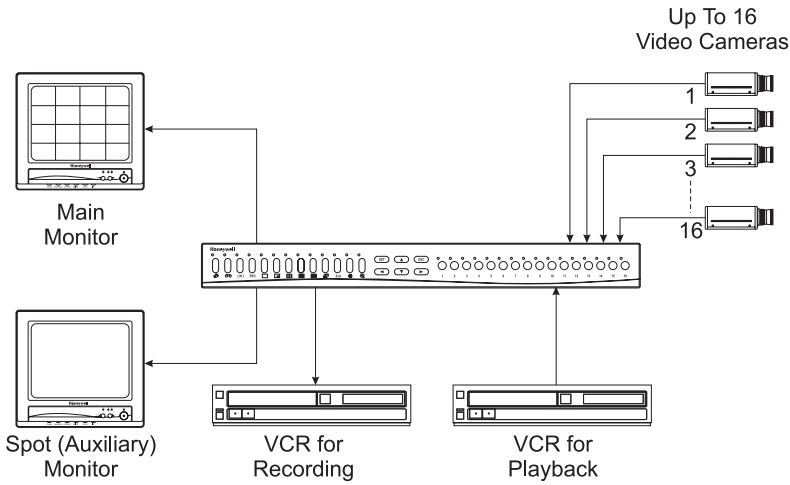
< Figure 1 > Typical multiplexer system configuration.
